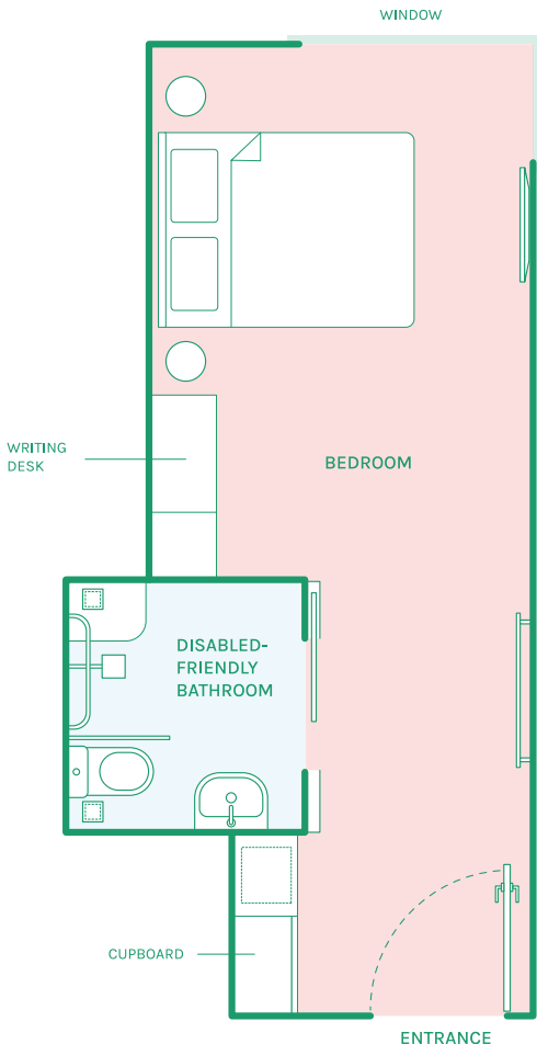
Studio Queen +
